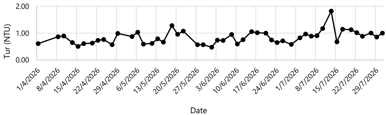
Turbidity (Ebb)
